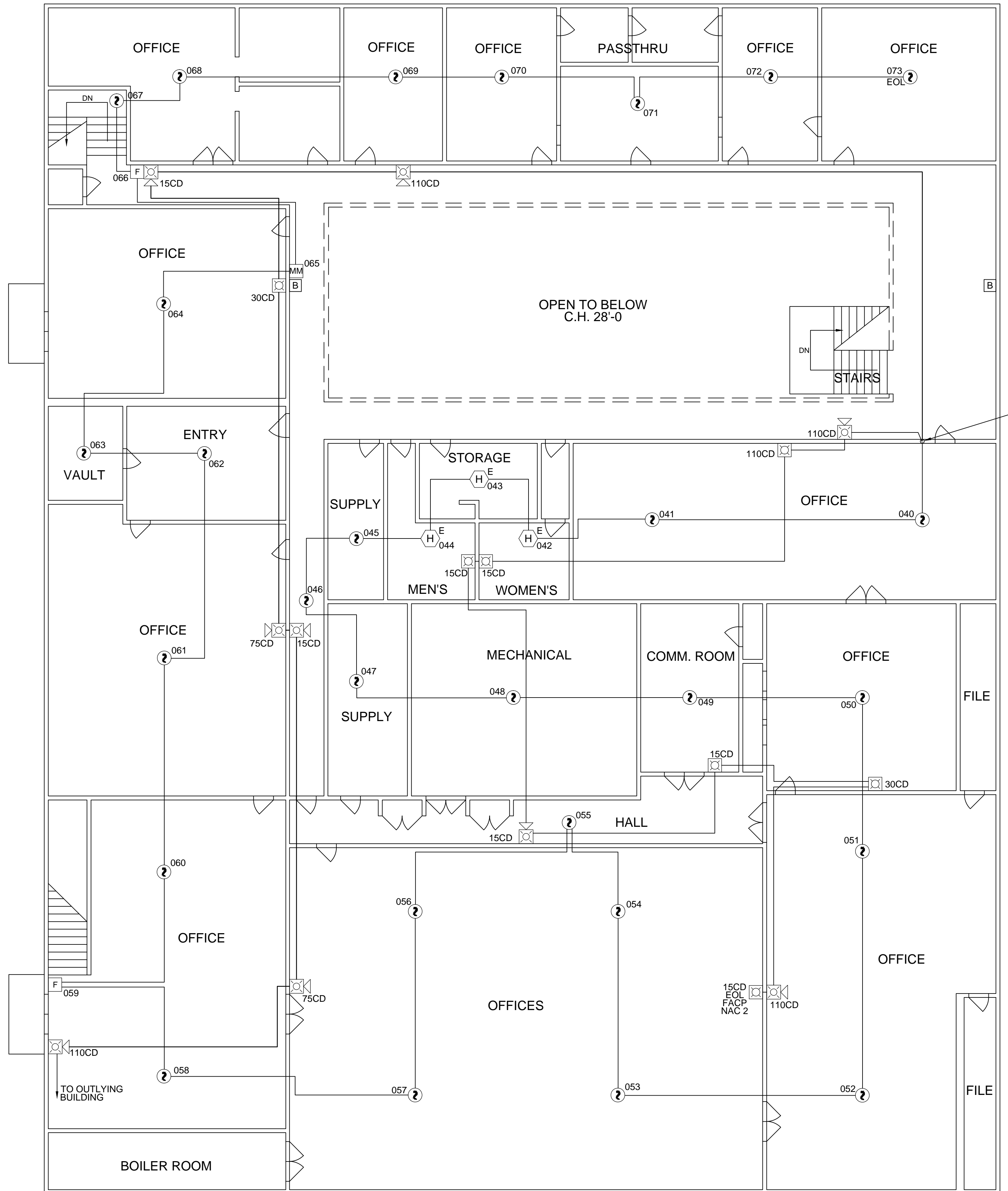
FIRE ALARM PLAN- UPPER LEVEL SCALE 1/8" = 1'-0"
